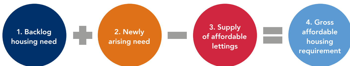
Figure 6.2 Model architecture
